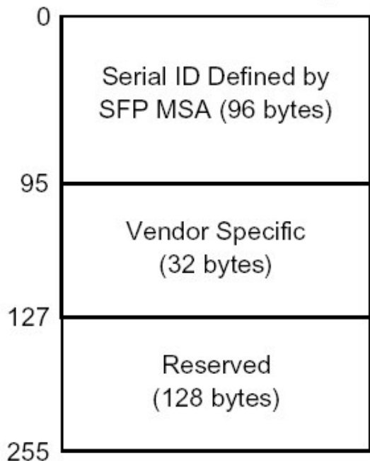
2 wire address 1010000x (A0h)
